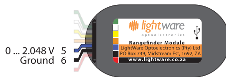
Figure 7 :: Analog voltage connections
